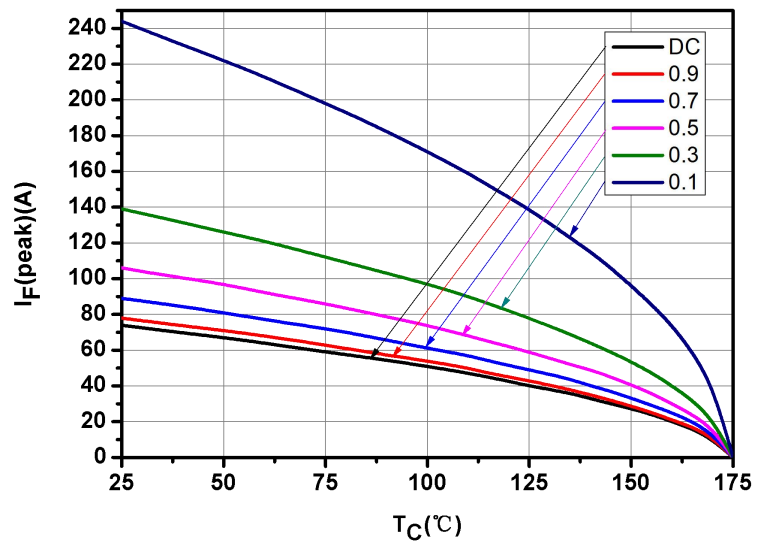
Fig.4-Current Derating
