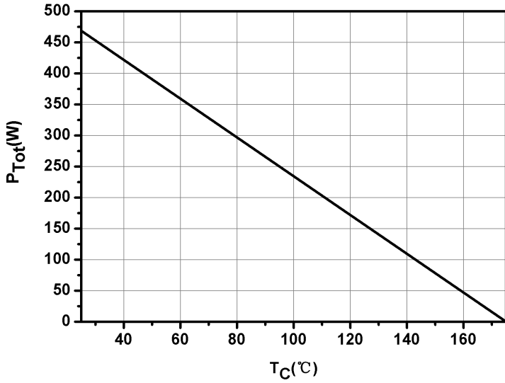
Fig.5-Power Derating
