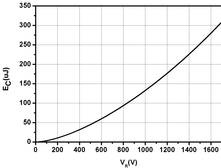
Fig.7-Capacitance Stored Energy
